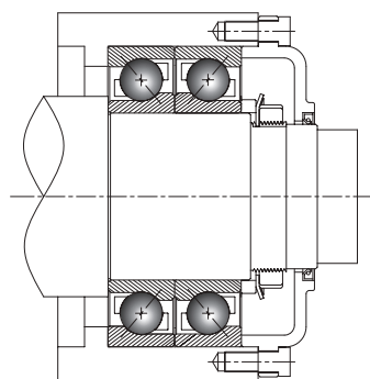
Figure 7. Montage face à face (DF).
