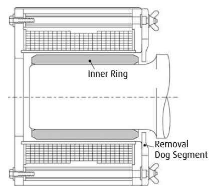
Removal of Inner Ring Using an Induction Heater
