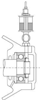
Drip Feed Lubrication: for high speeds
