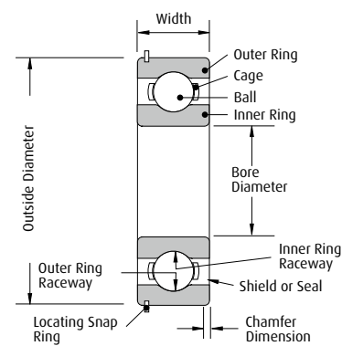
Single Row Deep Groove Ball Bearing
