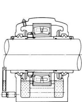
Oil Bath Lubrication: not for high speeds
