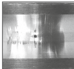
False Brinelling
