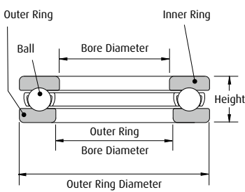
Single Direction Thrust Ball Bearing
