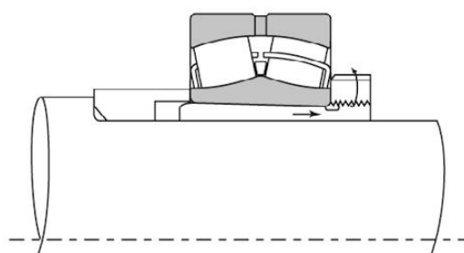
Mounting w/Adapter
