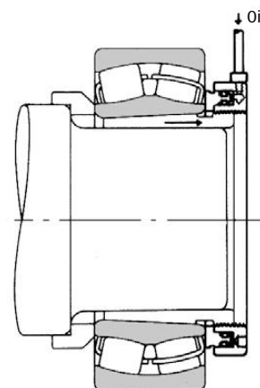
Removal Using a Hydraulic Nut
