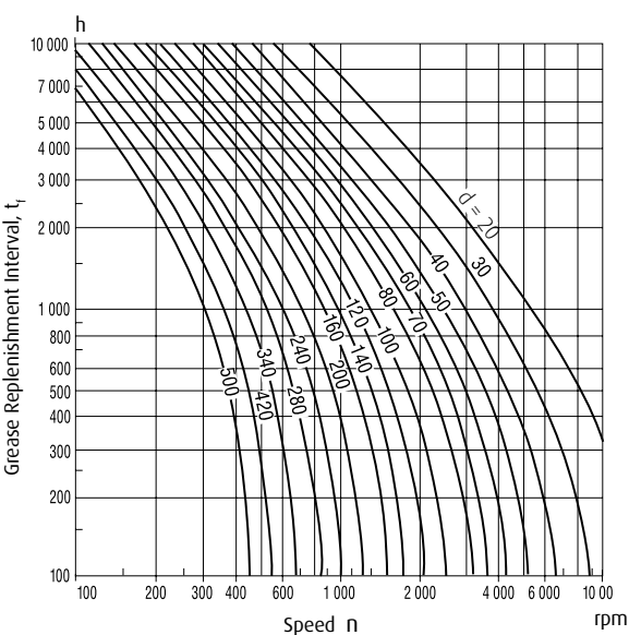
(2) Tapered Roller Bearings, Spherical Roller Bearings
