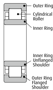
Cylindrical Roller Bearing (NU Style)
