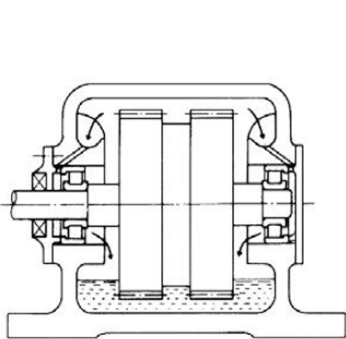
Splash Lubrication: gearboxes
