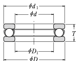
With Flat Seat
