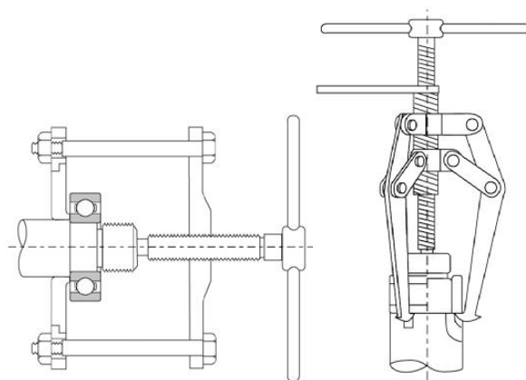
Removal of Inner Ring with Withdrawal Tools
