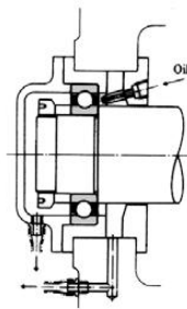
Jet Lubrication: ultra high speeds, like jet engine or machine tool spindles
