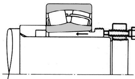
Mounting with Withdrawal Sleeve
