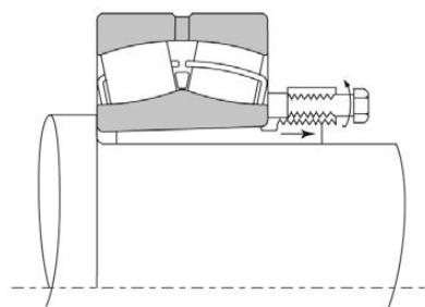
Removal of Withdrawal Sleeve with Withdrawal Nut
